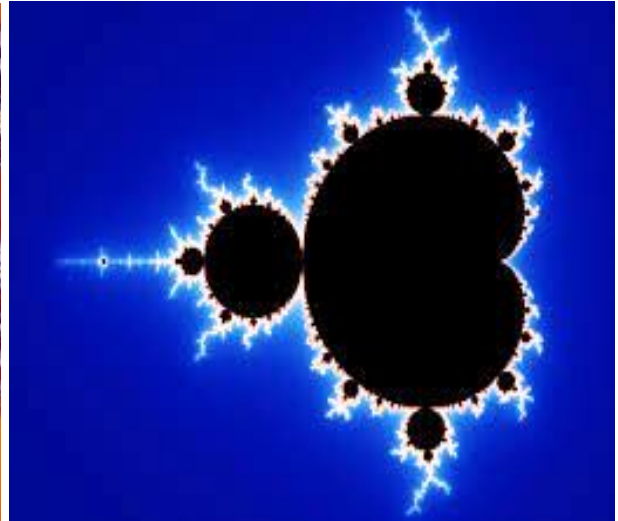
Mandelbrot Set
